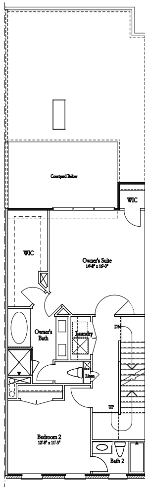
Second Floor With Optional 3rd Floor
